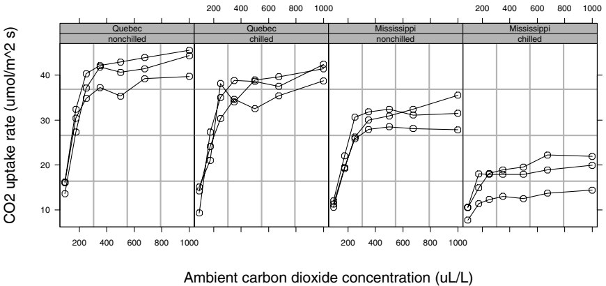
FIGURE 8.15. CO 2 uptake versus ambient CO 2 by treatment and type for Echinochloa crus-galli plants, 6 from Quebec and 6 from Mississippi. Half the plants of each type were chilled overnight before the measurements were taken.
