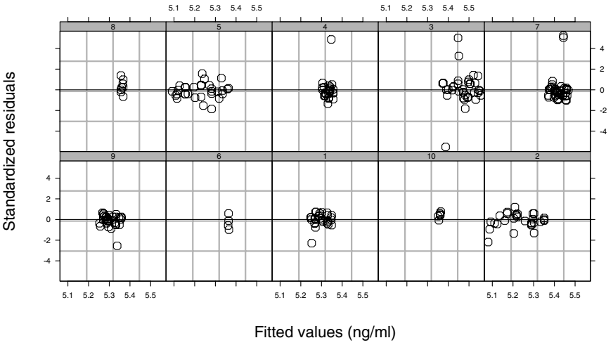
FIGURE 4.21. Scatter plots of standardized residuals versus fitted values for the fm2IGF.lme fit, by lot.
