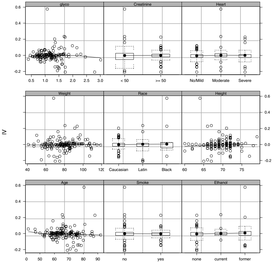
FIGURE 8.21. Estimated log-volume random effects from model fm1Quin.nlm versus demographic and physiological covariates in the quinidine data. A loess smoother is included in the scatter plots of the continuous covariates to aid in visualizing possible trends.
