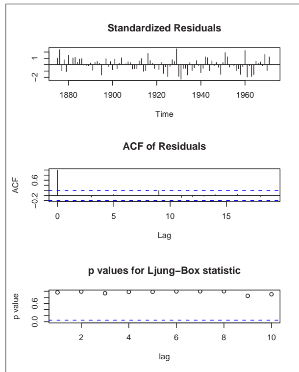
Figure 4.2: Output from tsdiag
